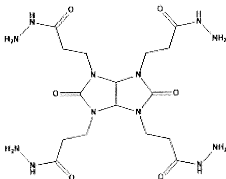
3,3',3'',3'''-(2,5-Dioxoimidazo[4,5-d]imidazole-1,3,4,6(2H,3aH,5H,6aH)-tetrayl)tetrapropanehydrazide
