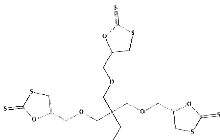
5,5'-(2-Ethyl-2-(((2-thioxo-1,3-oxathiolan-5-yl)methoxy)methyl)propane-1,3-diyl)bis(oxy)bis(methylene)bis(1,3-oxathiolane-2-thione)
