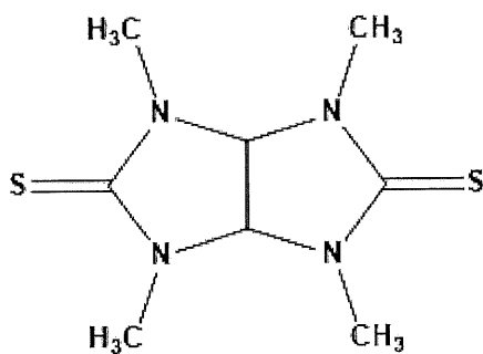
1,3,4,6-Tetramethyltetrahydroimidazo[4,5-d]imidazole-2,5(1H,3H)-dithione
